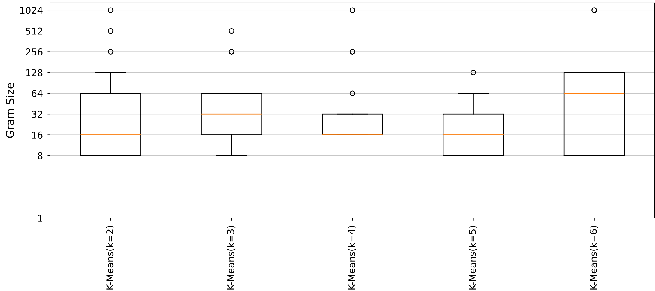
YARA Rules Gram Size Distribution (Cluster33_Size6 dataset)
